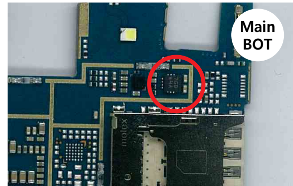
Accelerometer & Compass sensor
