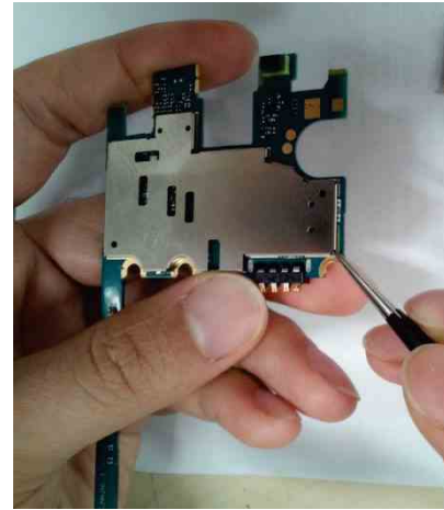
12. Take apart the Can shield(BOT)
