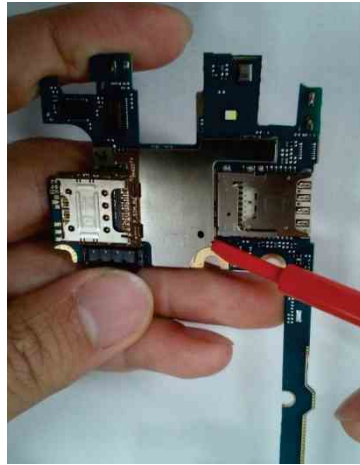
11. Take apart the Can shield(TOP)
