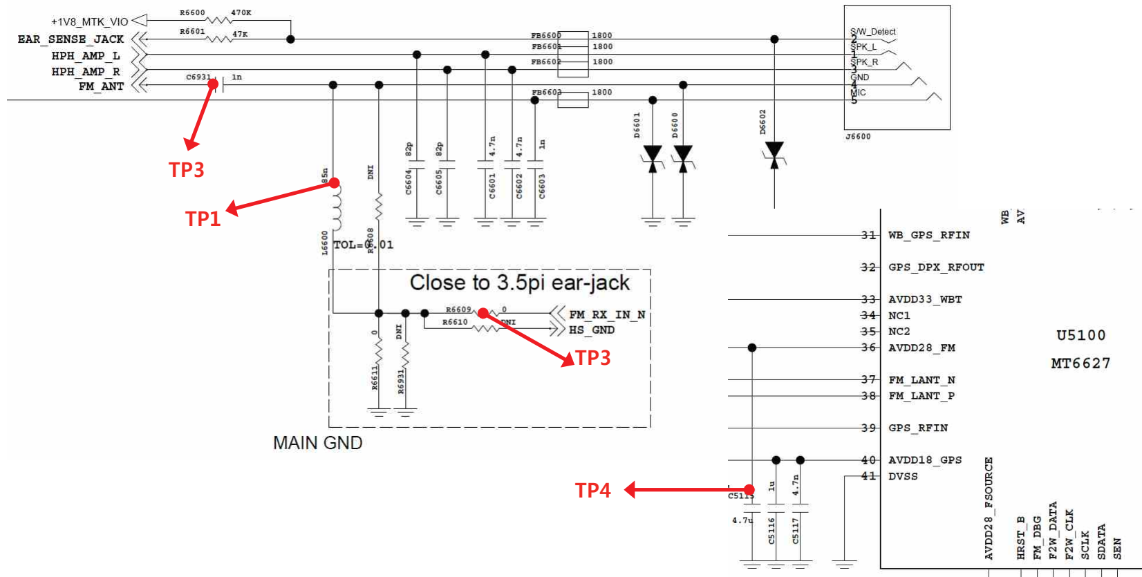
Circuit Diagram
