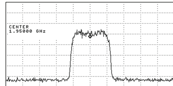
TP1_RF IN
